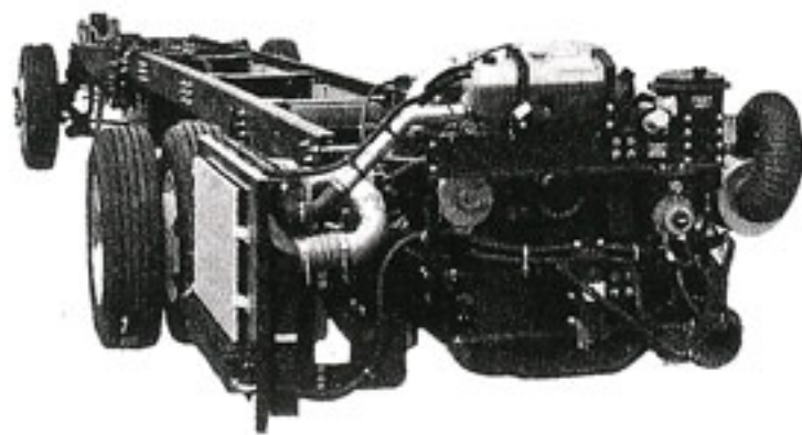
Freightliner Raised Rail 400 HP Cummins Diesel Pusher Chassis with side draft radiator and independent front suspension.
