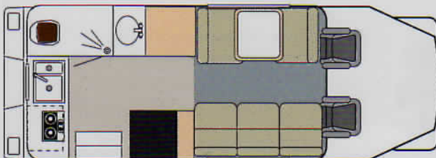
23' Rear kitchen w/sofa and dinette
