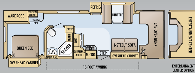
33DS Chevy® Kodiak C5500 Chassis
